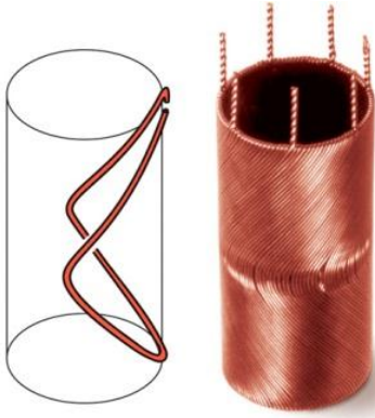
Figure 5 The heart of the maxon motors is the worldwide patented ironless winding. This motor principle offers unique advantages; no magnetic detent and low electromagnetic disturbances. Its efficiency of up to 90% surpasses other motor systems by far. © 2010 maxon motor
